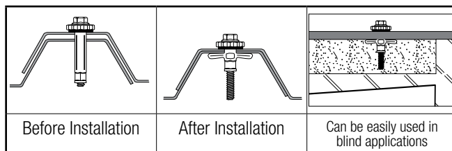
Carbon Steel Screw: Elco Flag
