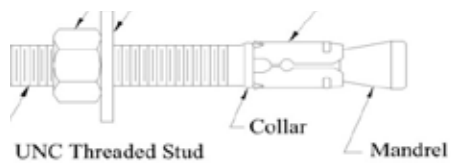
FIGURE 1—US ANCHOR ULTRAWEDGE+ WEDGE ANCHOR COMPONENTS
